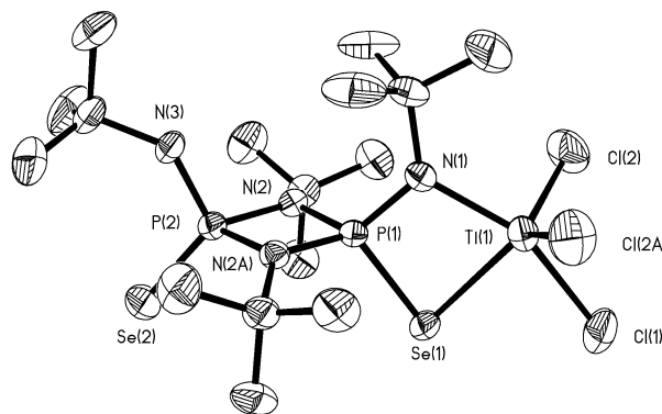
Fig. 4 Solid-state structure of 10 . The solvent molecule (toluene) is not shown. The disulfur complex ( 9 ) is isostructural.
