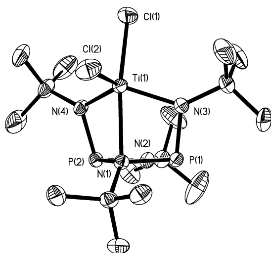
Fig. 1 Solid-state structure of 2 .
