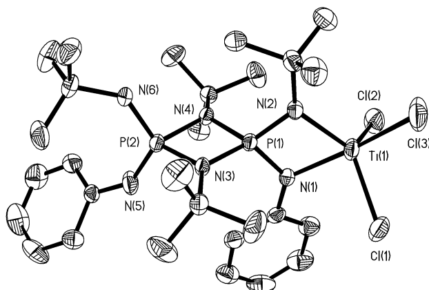
Fig. 3 Solid-state structure of 5 . The solvent molecule (toluene) is not shown.
