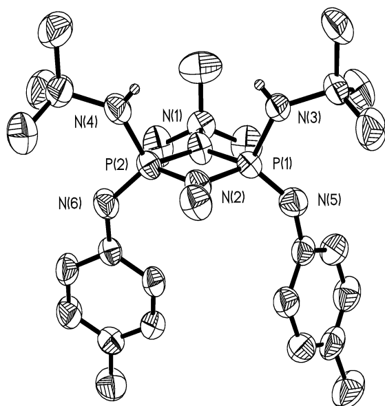
Fig. 2 Solid-state structure of 4 . The proximal tert -butyl group has been truncated to the quaternary carbon for clarity. Compound 3 has a similar structure.
